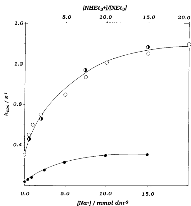
Fig. 3 Kinetics for the reaction between [\text{Fe}_4\text{S}_4(\text{SPh})_4]^{2-} (0.1 \text{mmol dm}^{-3} ) and \text{Et}_2\text{NCS}_2^- in MeCN at 25.0 °C. The bottom curve illustrates the effect of \text{Na}^+ on the rate of the reaction ( \bullet ); the curve is that defined by equation (3). The top curve shows the combined effect of \text{Na}^+ and \text{H}^+ ; data points correspond to: [\text{NHEt}_3^+] = 10 \text{ mmol dm}^{-3} ( \circ ), [\text{NHEt}_3^+] = 20 \text{ mmol dm}^{-3} ( \bullet ); [\text{Et}_2\text{NCS}_2^-] = 2.0 \text{ mmol dm}^{-3} , [\text{NEt}_3] = 1\text{--}20 \text{ mmol dm}^{-3} . The curve is that defined by equation (6).
